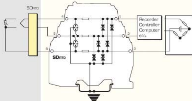
3-wire RTDs
