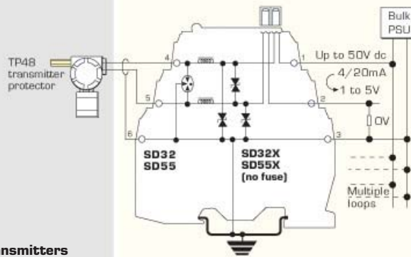
2-wire transmitters
