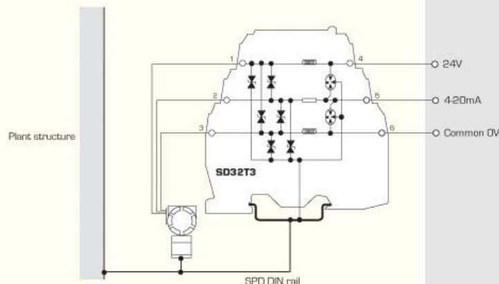
3-wire transmitter or sensor
