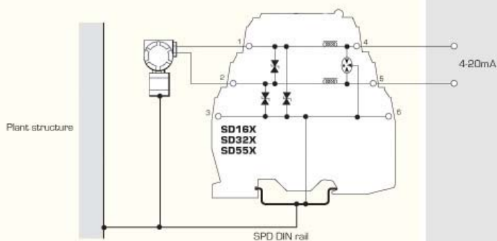
2-wire transmitter or sensor
