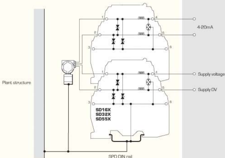
4-wire transmitter or sensor
