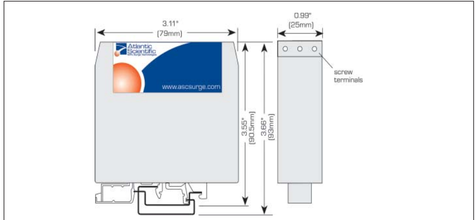
Figure 1 Dimensions
